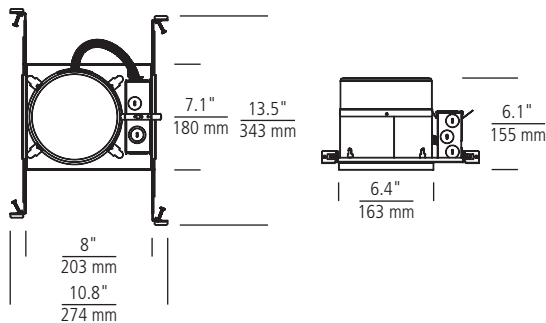
11019 New Construction / IC / Shallow Airtight
